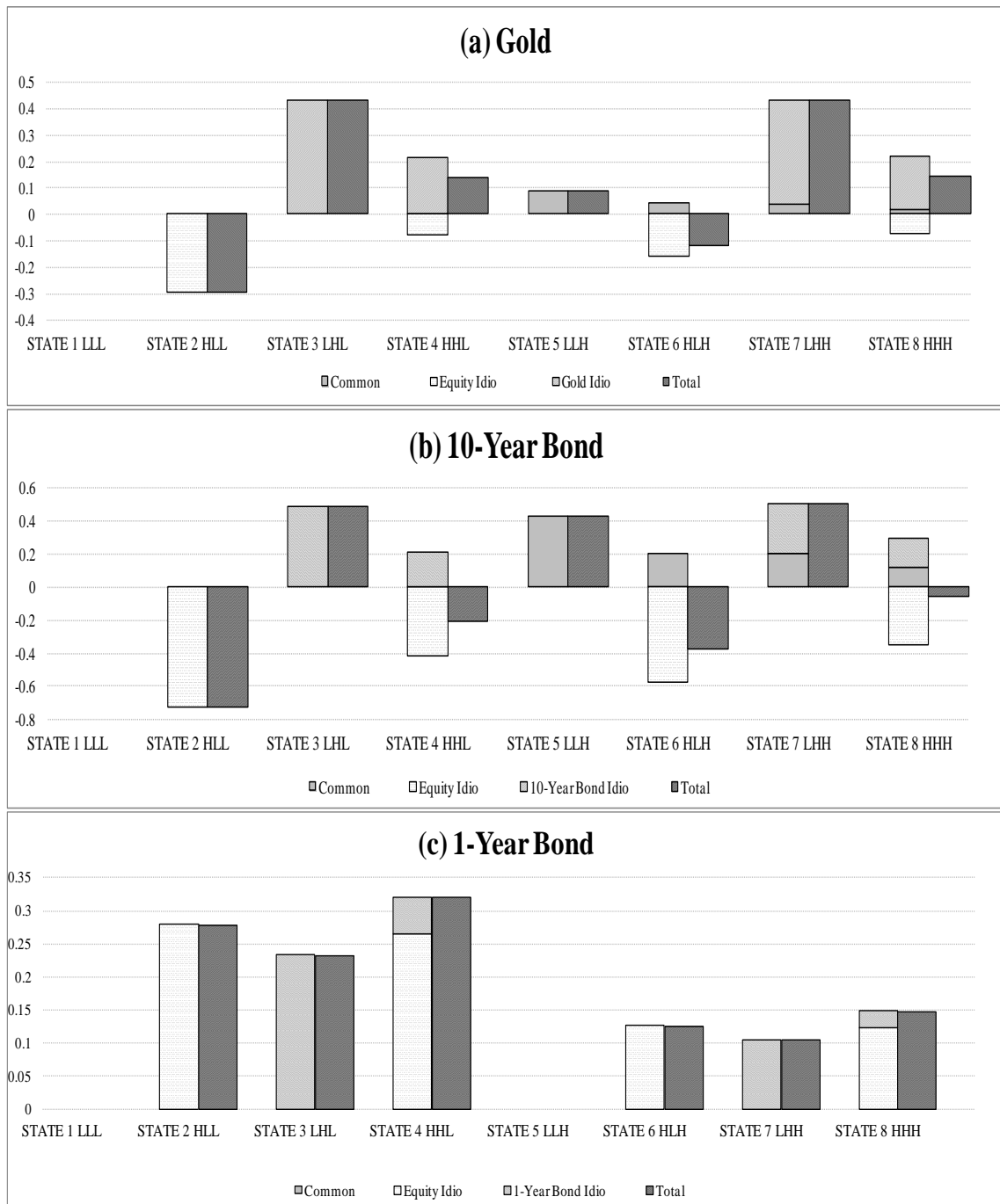
Figure 7: Decomposition of equity correlation with (a) Gold, (b) 10-Year Bond & (c) 1-Year Bond by shock and state.
