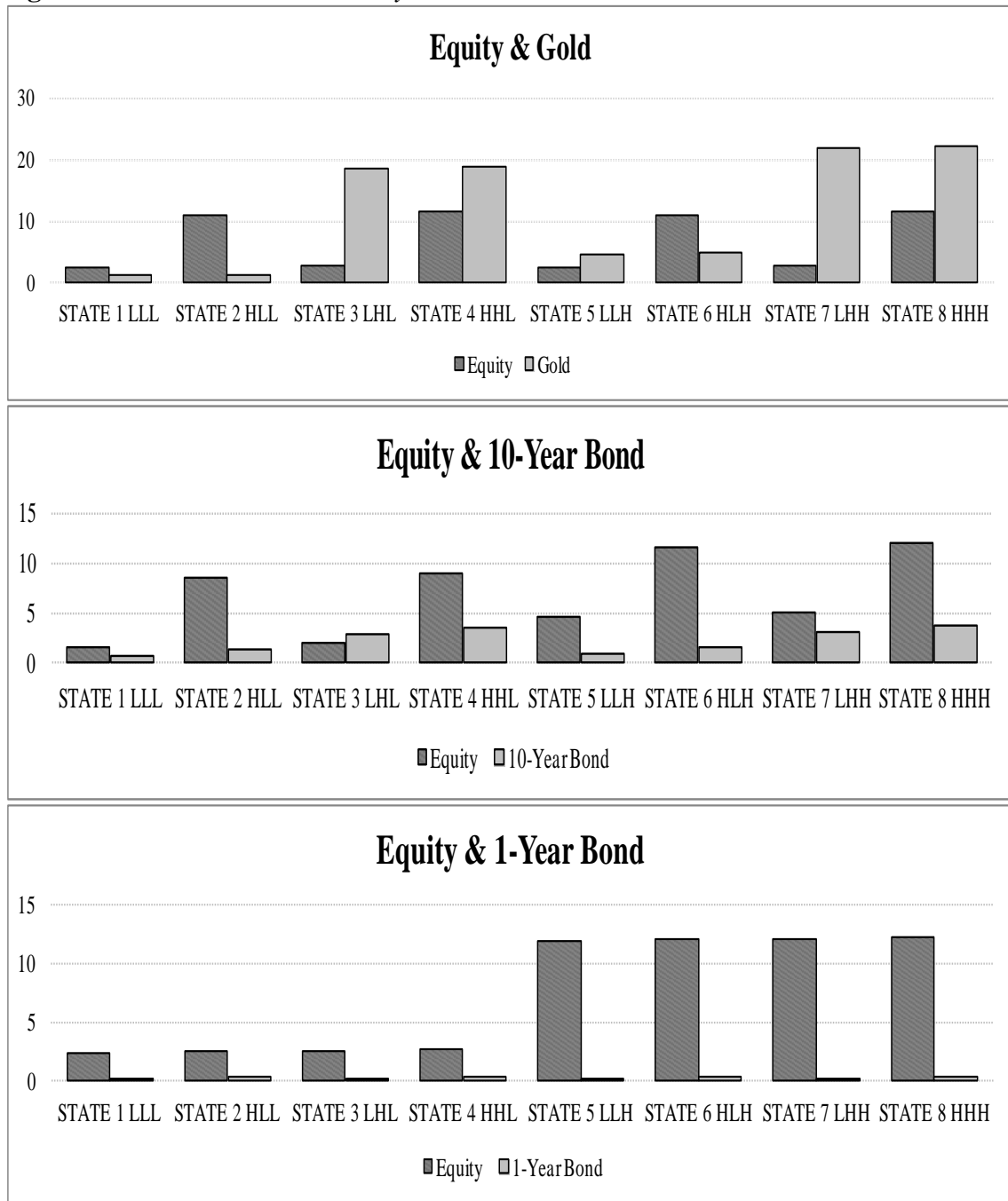
Figure 4: Conditional variances by state
