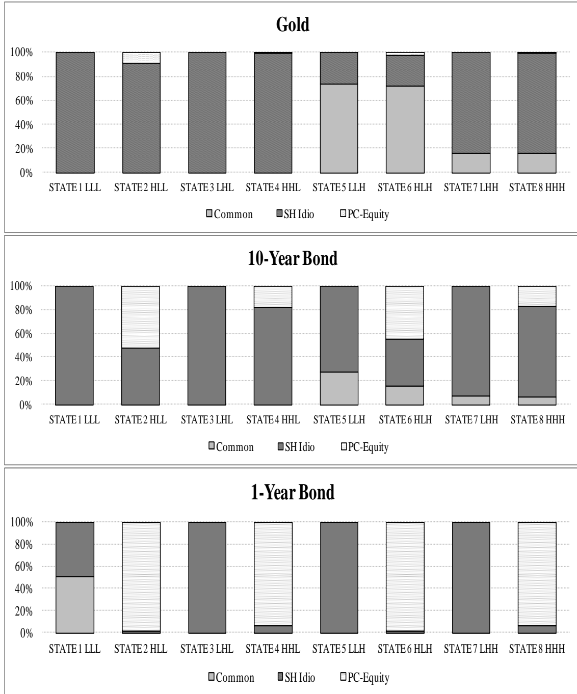
Figure 6: Decomposition of variance of safe haven asset return by State
