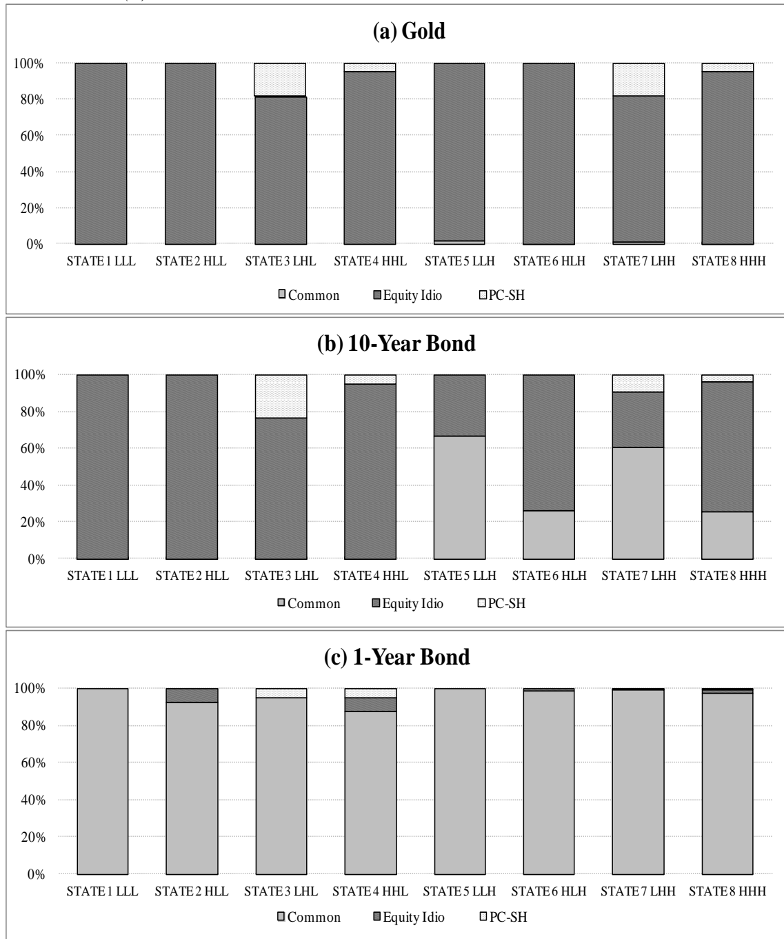
Figure 5: Decomposition of equity variance by state in pairings with (a) Gold, (b) 10-Year Bond & (c) 1-Year Bond
