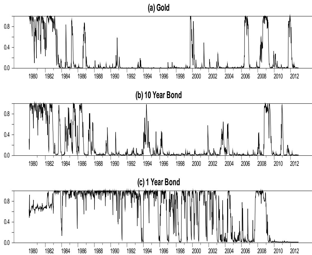
Figure 3: Filter probabilities of safe haven idiosyncratic shock being in high-volatility regime.
