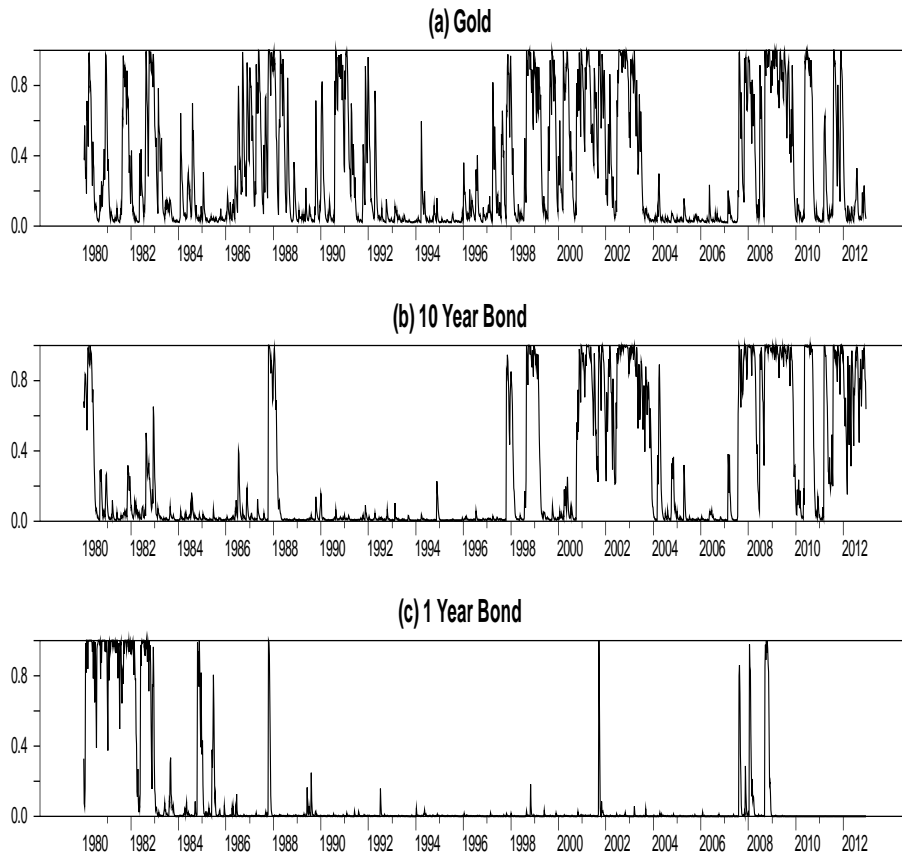
Figure 2: Filter probabilities of equity idiosyncratic shock being in the high-volatility regime in pairing with (a) Gold, (b) 10-Year Bond, (c) 1-Year Bond
