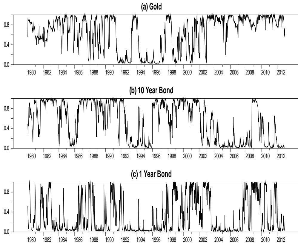
Figure 1: Filter probabilities of high-volatility common shocks between equity and: (a) Gold, (b) 10-Year Bond, (c) 1-Year Bond
